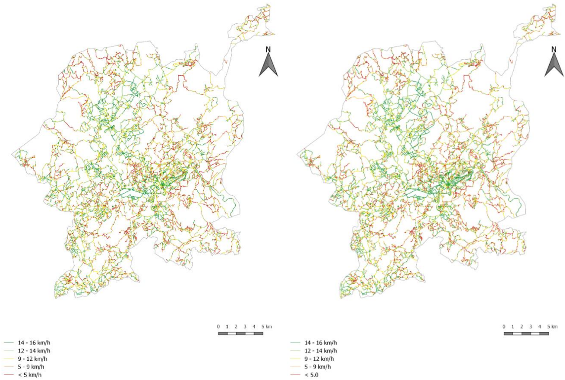
Figure 176 – Cycling Speeds in the Road Network of Guimarães considering slopes, cycling infrastructure, road hierarchy and accidents for the current scenario.
